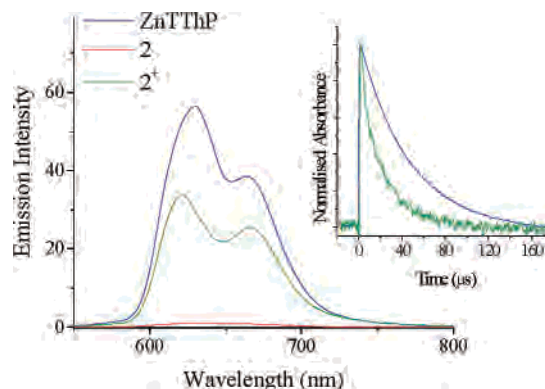
Figure 4. Fluorescence spectra for ZnTThP, 2 , and 2^+ (in ethanol). Inset: Normalized transient absorption decay traces of ZnTThP ( ^3\tau = 40 \mu\text{s} ) and 2^+ ( ^3\tau = 20 \mu\text{s} ) at 490 nm ( \lambda_{\text{exc}} = 532 \text{ nm} ; 1 atm of argon).
